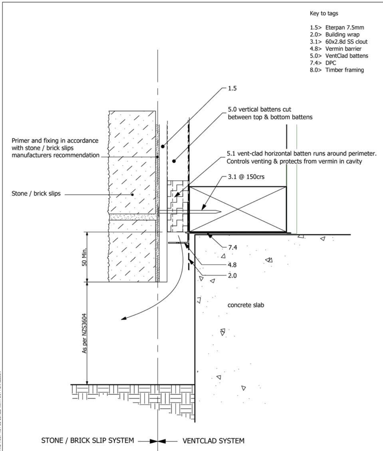
Vertical section through sill at slab
